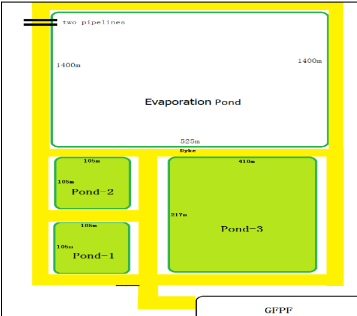
Figure 1: Gummry Burrow Pits Ponds and Evaporation Pond Layout
